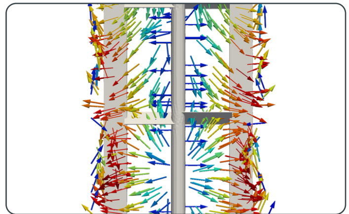
FLOW LINES | ANCHOR IMPELLER REPRESENTATION
