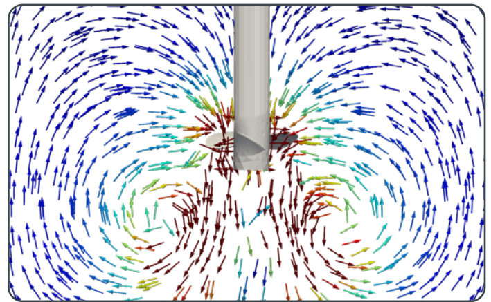
FLOW LINES | MARINE IMPELLER REPRESENTATION
