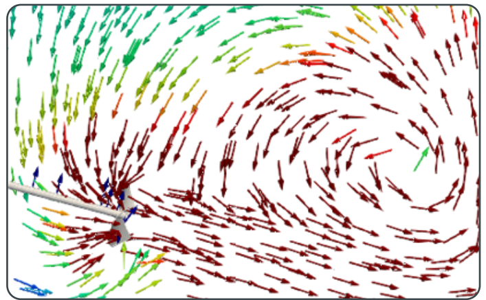
FLOW LINES | SABRE IMPELLER REPRESENTATION
