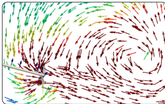
FLOW LINES | SABRE IMPELLER REPRESENTATION
