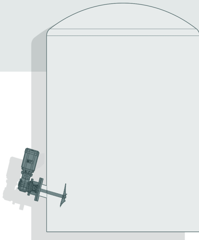
FLOW LINES | SABRE IMPELLER REPRESENTATION
