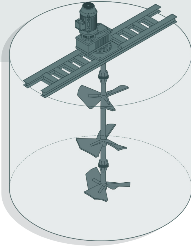
FLOW LINES | SABRE IMPELLER REPRESENTATION
